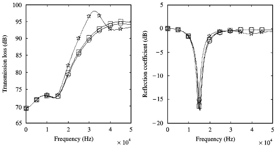
Figure 11. Transmission loss and reflection coefficients with different azimuthal angles for the sandwich plate (filler B): \circ – \circ –, 0^\circ ; \square – \square –, 45^\circ ; \star – \star –, 90^\circ ; incident angle = 50^\circ ( t_c = 0.01 m, t_p = 0.005 m, water–air).
