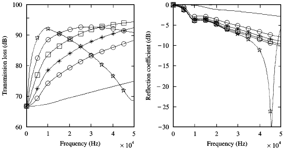
Figure 6. Transmission loss and reflection coefficients with various thickness of base plate for coating layer above: —, t_p = 0 ; \circ-\circ , t_c = 0.005 m; \star-\star , t_p = 0.01 m; \square-\square , t_p = 0.02 m; \diamond-\diamond , t_p = 0.04 m; \star-\star , t_p = 0.1 m. ( t_c = 0.01 m, water-air).
