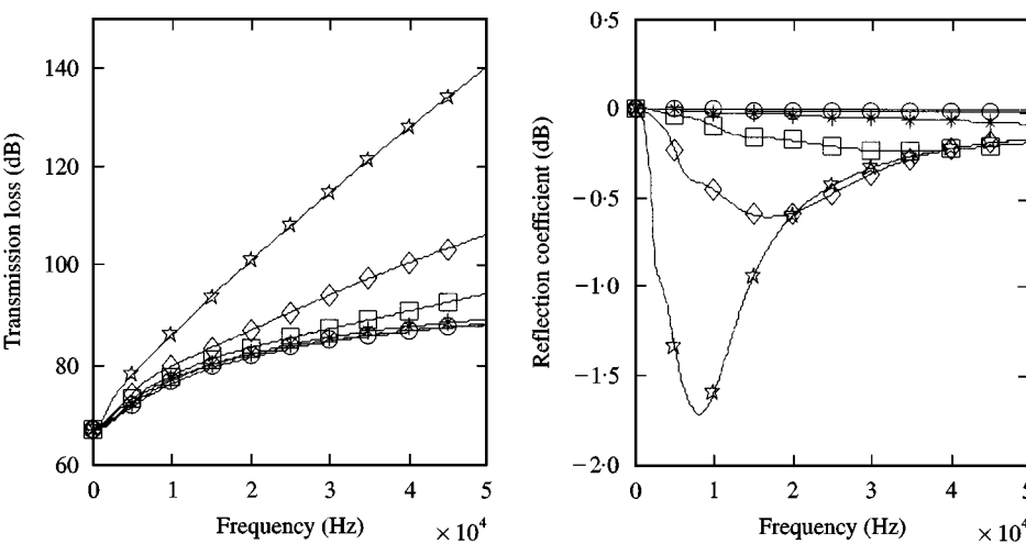
Figure 5. Transmission loss and reflection coefficients with various thickness of coating layer for coating layer below: —, t_c = 0 ; \circ — \circ —, t_c = 0.005 m; \star — \star —, t_c = 0.01 m; \square — \square —, t_c = 0.02 m; \diamond — \diamond —, t_c = 0.04 m; \star — \star —, t_c = 0.1 m. ( t_p = 0.01 m, water-air).
