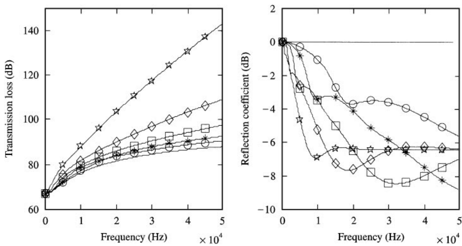
Figure 4. Transmission loss and reflection coefficients with various thickness of coating layer for coating layer above: —, t_c = 0 ; \circ — \circ —, t_c = 0.005 m; \star — \star —, t_c = 0.01 m; \square — \square —, t_c = 0.02 m; \diamond — \diamond —, t_c = 0.04 m; \star — \star —, t_c = 0.1 m. ( t_p = 0.01 m, water-air).
