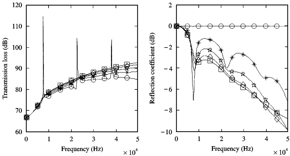
Figure 9. Transmission loss and reflection coefficients with different damping factors for coating layer above: -\bigcirc-\bigcirc- , \eta = 0 ; -\star-\star- , \eta = 0.2 ; -\triangle-\triangle- , \eta = 0.4 ; -\diamond-\diamond- , \eta = 0.6 ; -\square-\square- , \eta = 0.8 ; ( t_c = t_p = 0.1 m, water-air).
