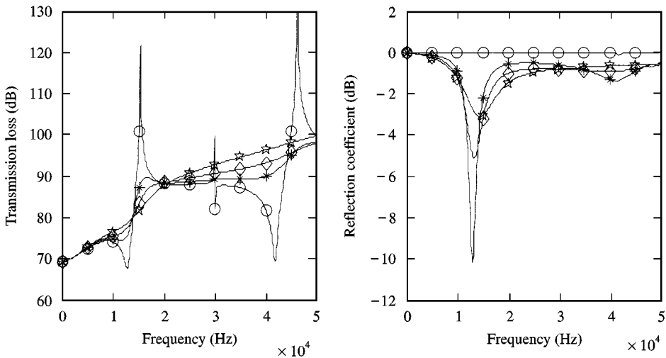
Figure 10. Transmission loss and reflection coefficients with different damping factors of filler A for the sandwich plate. -\bigcirc-\bigcirc- , \eta = 0 ; -\star-\star- , \eta = 0.2 ; -\diamond-\diamond- , \eta = 0.4 ; -\triangle-\triangle- , \eta = 0.8 . incident angle = 50^\circ ( t_c = 0.01 m, t_p = 0.005 m, water-air).
